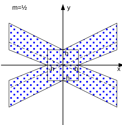
Figure 13: Hysteresis in low asymmetrical mode
